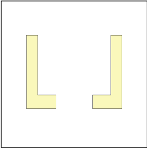
Step Markers Aluminum Right and Left Pair DIMENSIONS: 1"Dx3"Wx9"H SKU: GBC-1130
